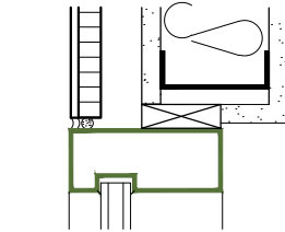
4A WINDOW HEAD - FLUSH
