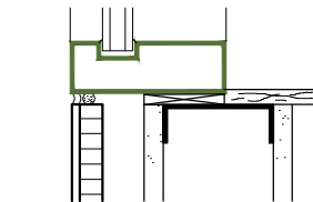
3A WINDOW SILL - FLUSH
