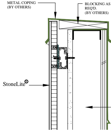
5A METAL COPING DETAIL
