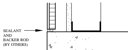
1A BASE DETAIL
