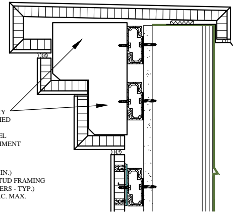
5B STONE PANEL CORNICE
