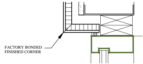
4B WINDOW HEAD - RECESSED
