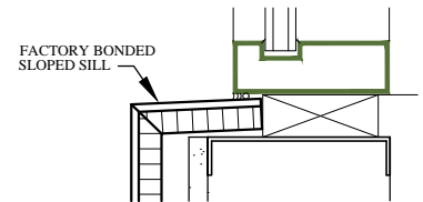
3B WINDOW SILL - RECESSED
