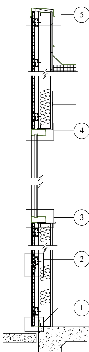
WALL SECTION
