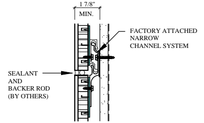
2B NARROW JOINT CHANNEL SYSTEM
