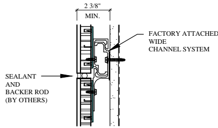
2A WIDE JOINT CHANNEL SYSTEM
