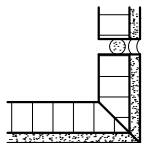
FINISHED RETURN & CAULK JOINT
