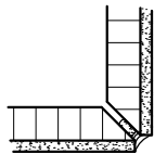
QUIRK MITER CORNER
