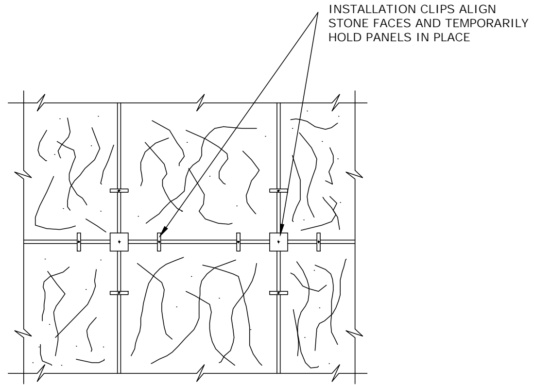
TYPICAL ELEVATION
